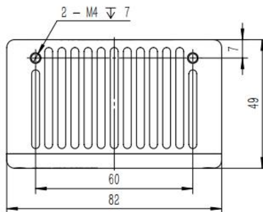
Left View of HPS-3D640
